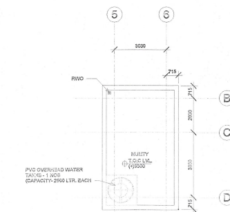
4 MUMTY PLAN 1:100
