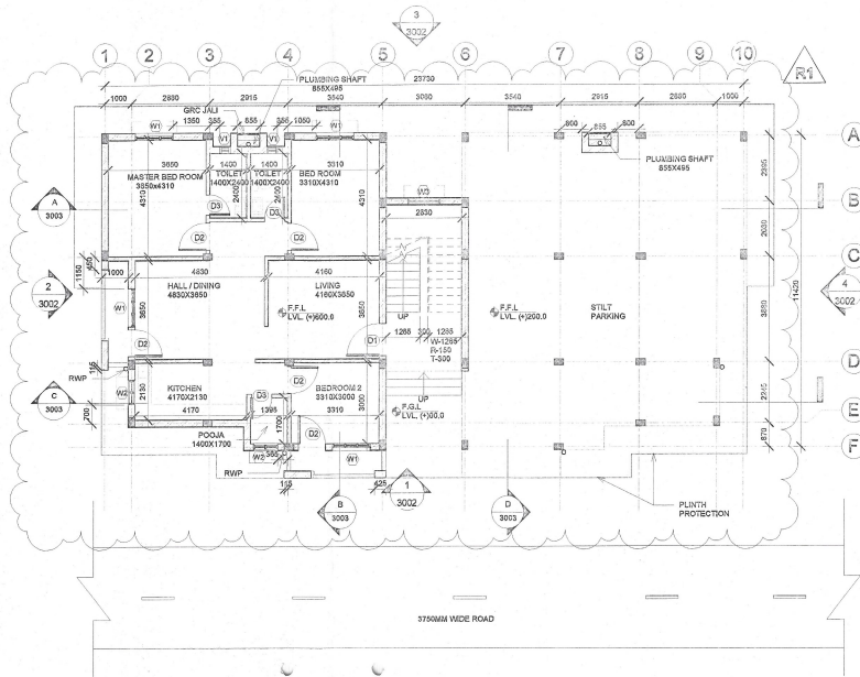
1 GROUND FLOOR PLAN 1:100
